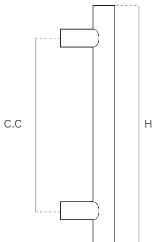
● AÇO INOX SATINADO IN.07.286.D.25 ASA DUPLA H:450 mm | C.C.: 300 mm Ref: 206401016300 H:600 mm | C.C.: 450 mm Ref: 206401022006
